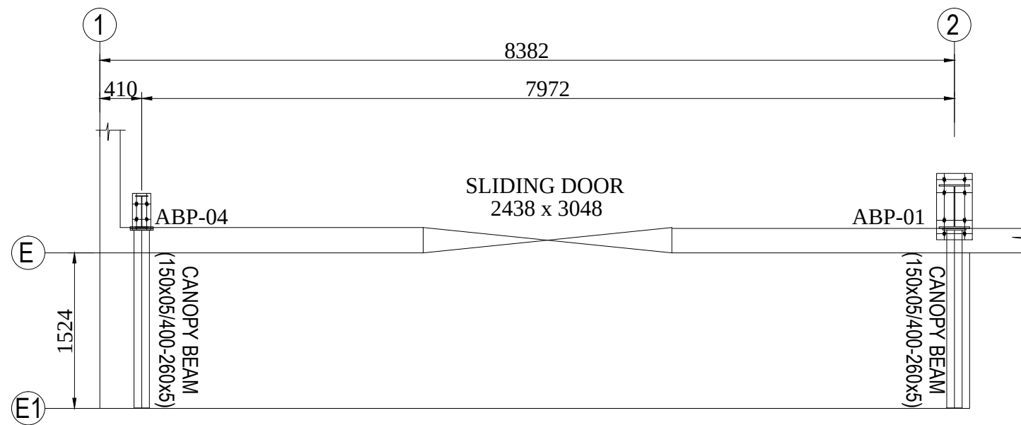
CANOPY LAYOUT PLAN
