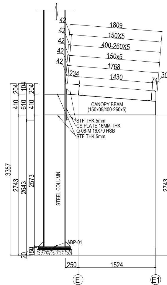
CANOPY CROSS SECTION @ 02 DETAIL (B-B)
