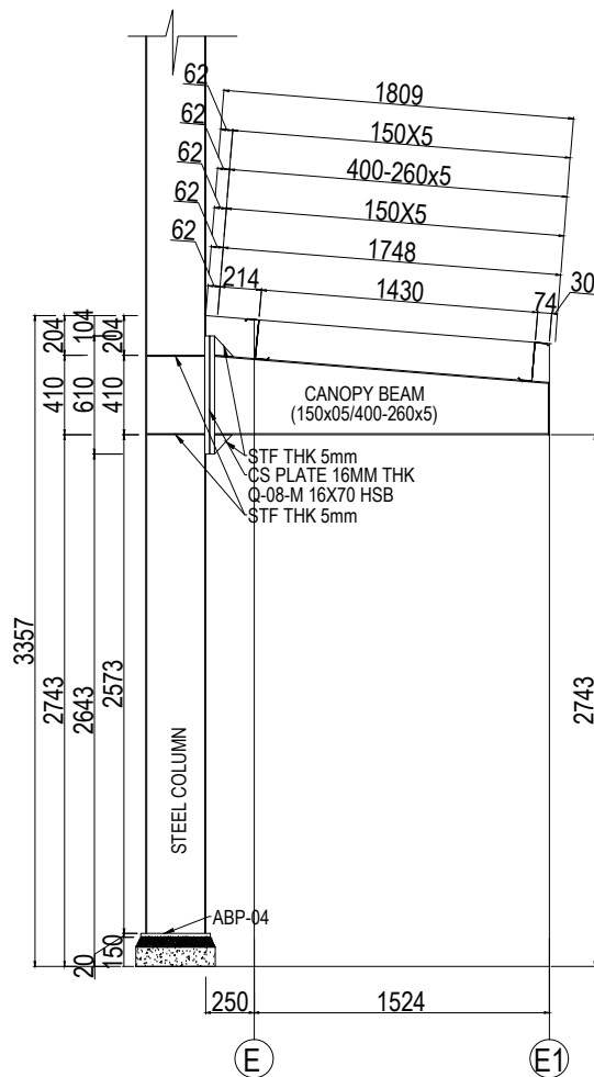
CANOPY CROSS SECTION @ 01 DETAIL (A-A)
